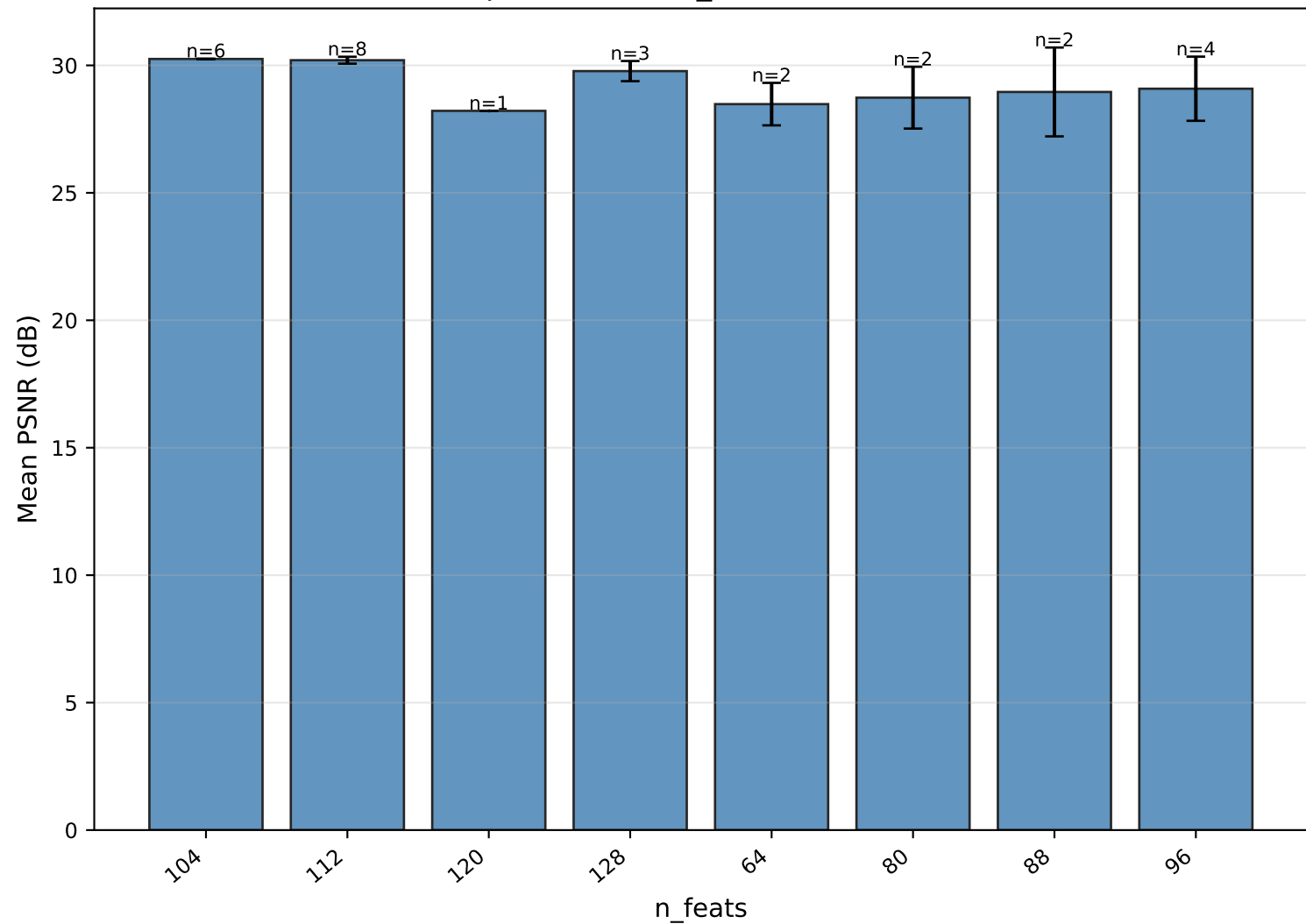
Mean PSNR per value of n_feats — WaveletAttention
